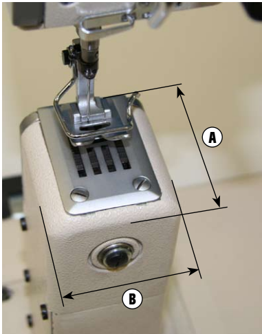
A size 64 mm B size 57 mm
