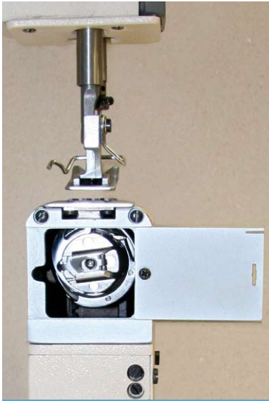
Machine is equipped with extra large diameter of hook.
